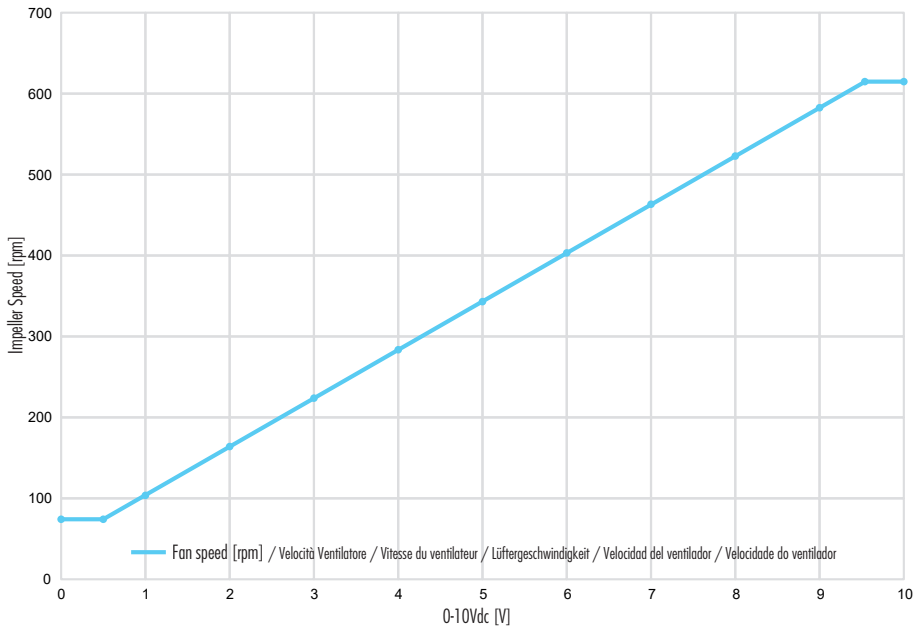
Speed Vs Voltage
