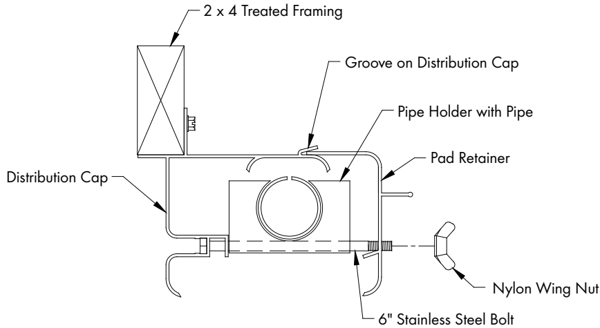
Figure 17A Standard Pad Retainer
