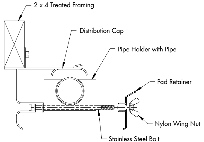
Figure 17B Open Header Pad Retainer
